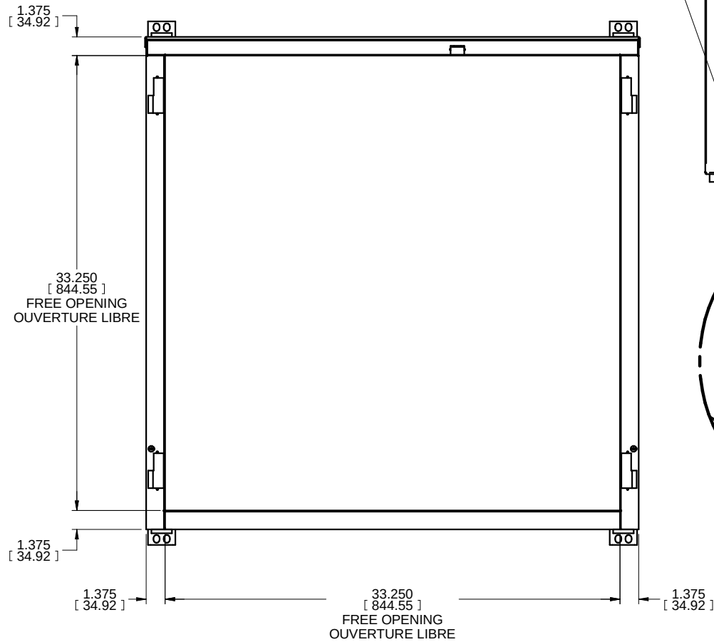
DETAIL D
