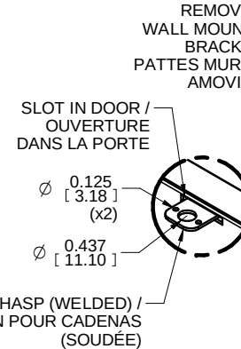
DETAIL G
