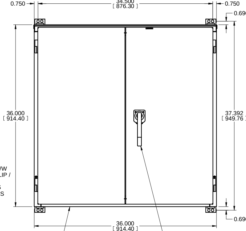
FRONT / FACE
