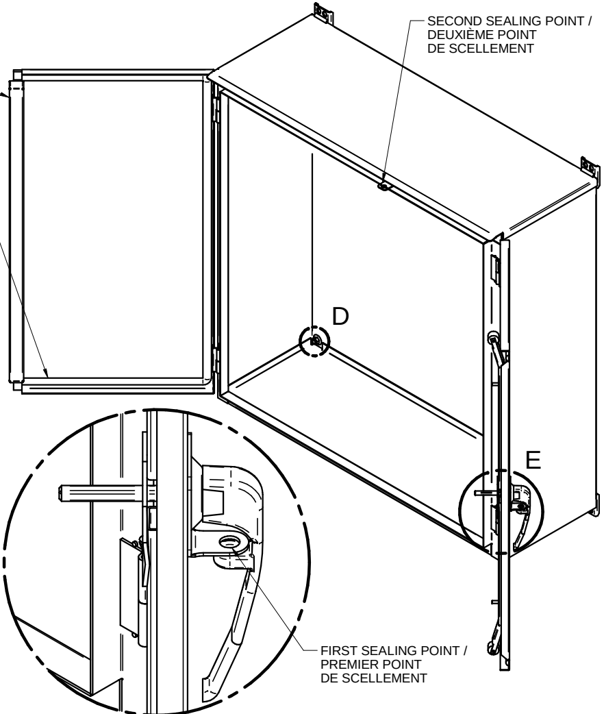
DETAIL E
