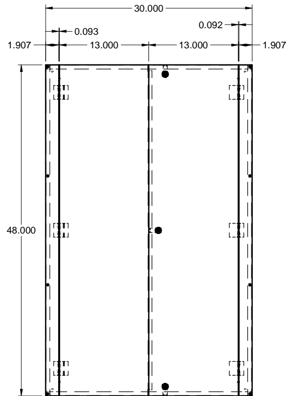
FRONT / FACE
