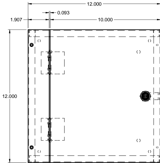
FRONT / FACE
