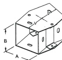
Coude 22.5°
