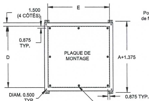
Section W-W
