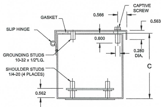
Section Y-Y
