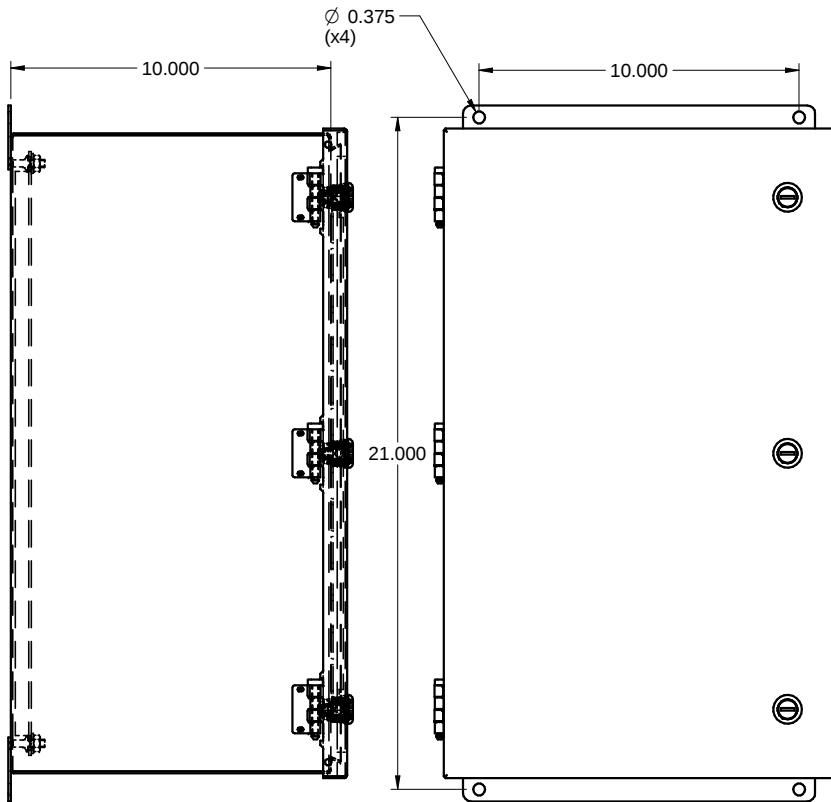
FRONT / FACE
