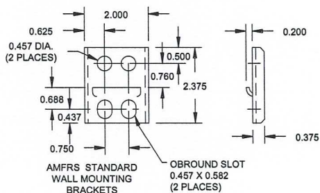
WALL MOUNTING BRACKETS POSITION FOR ALL MODELS (ALL 4 CORNERS)
