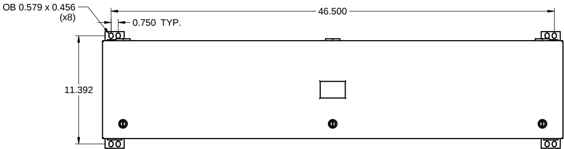
FRONT / FACE
