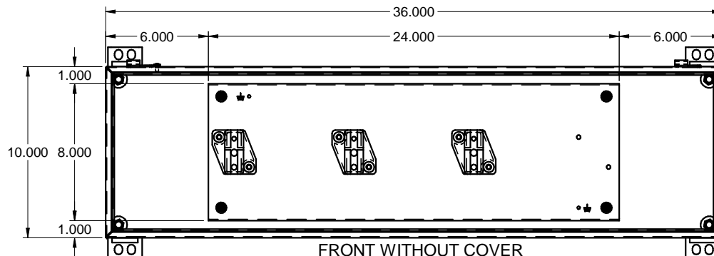
FRONT WITHOUT COVER / FACE SANS COUVERCLE
