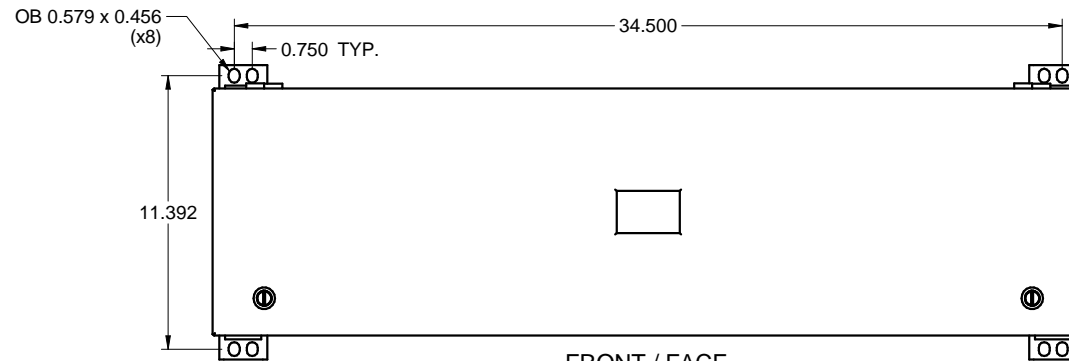
FRONT / FACE
