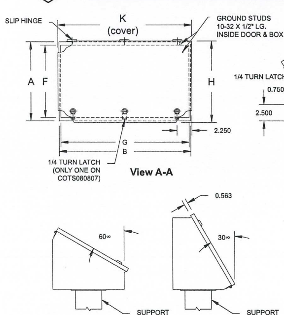
Mounting Options
