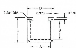
2-1/2" x 2-1/2" & 4" x 4" MODEL
