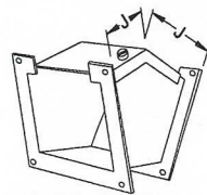
45 elbow outside opening
