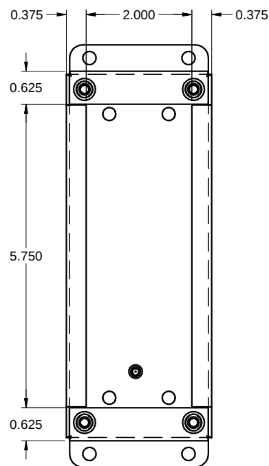
FRONT without door / FACE sans couvercle
