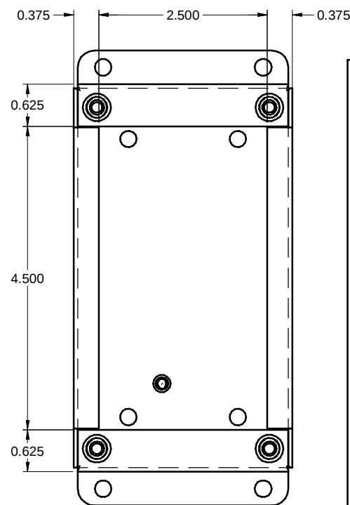
FRONT without door / FACE sans couvercle
