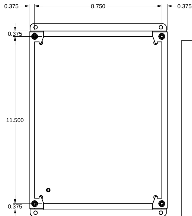
FRONT without door / FACE sans couvercle
