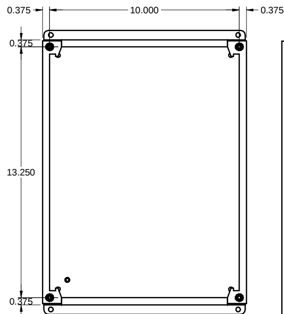
FRONT without door / FACE sans couvercle
