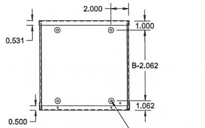
Front View WITHOUT COVER
