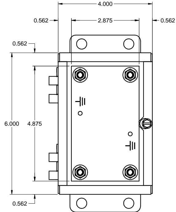
FRONT WITHOUT COVER / FACE SANS COUVERCLE
