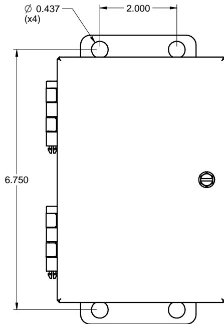
FRONT / FACE
