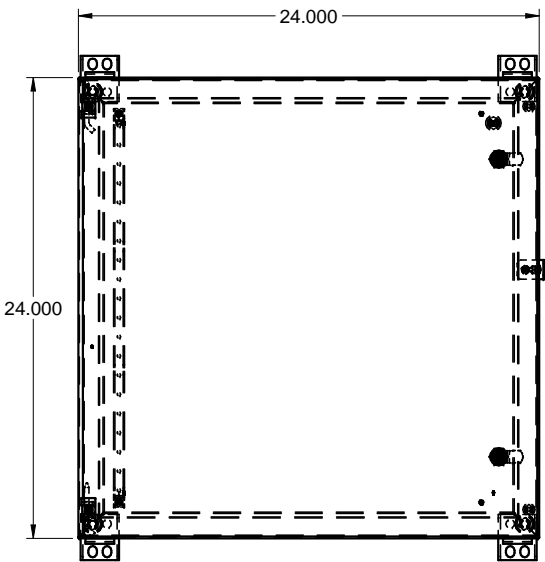
FRONT / FACE
