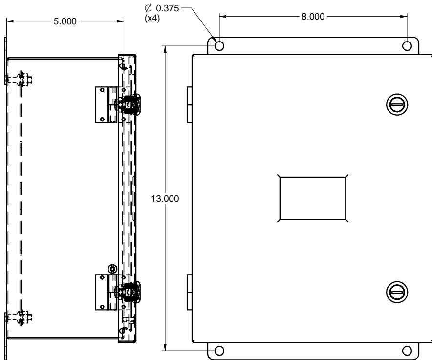
FRONT / FACE
