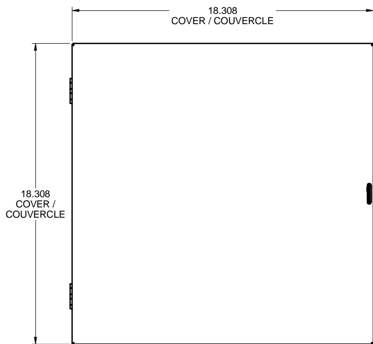
FRONT / FACE
