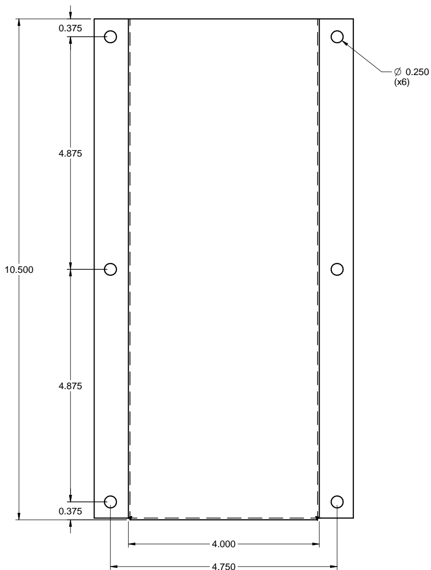
FRONT / FACE
