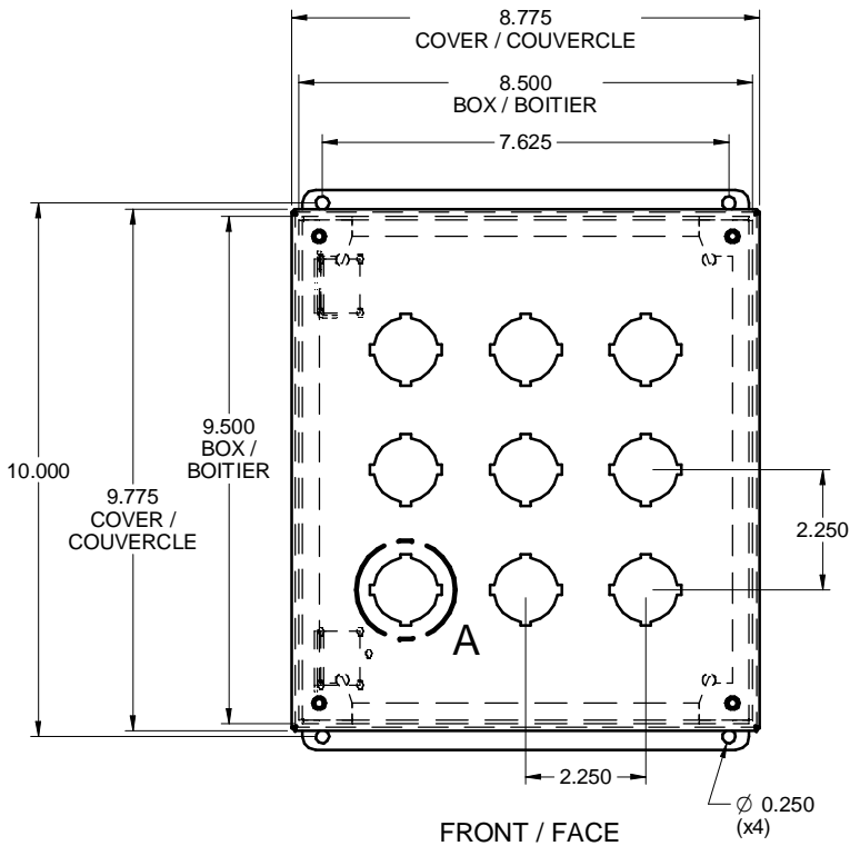
FRONT / FACE
