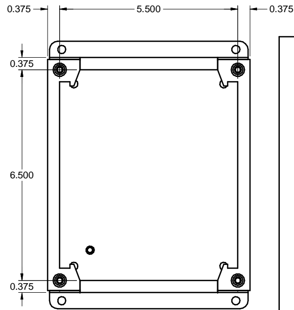
FRONT without door / FACE sans couvercle
