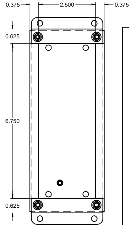
FRONT without door / FACE sans couvercle
